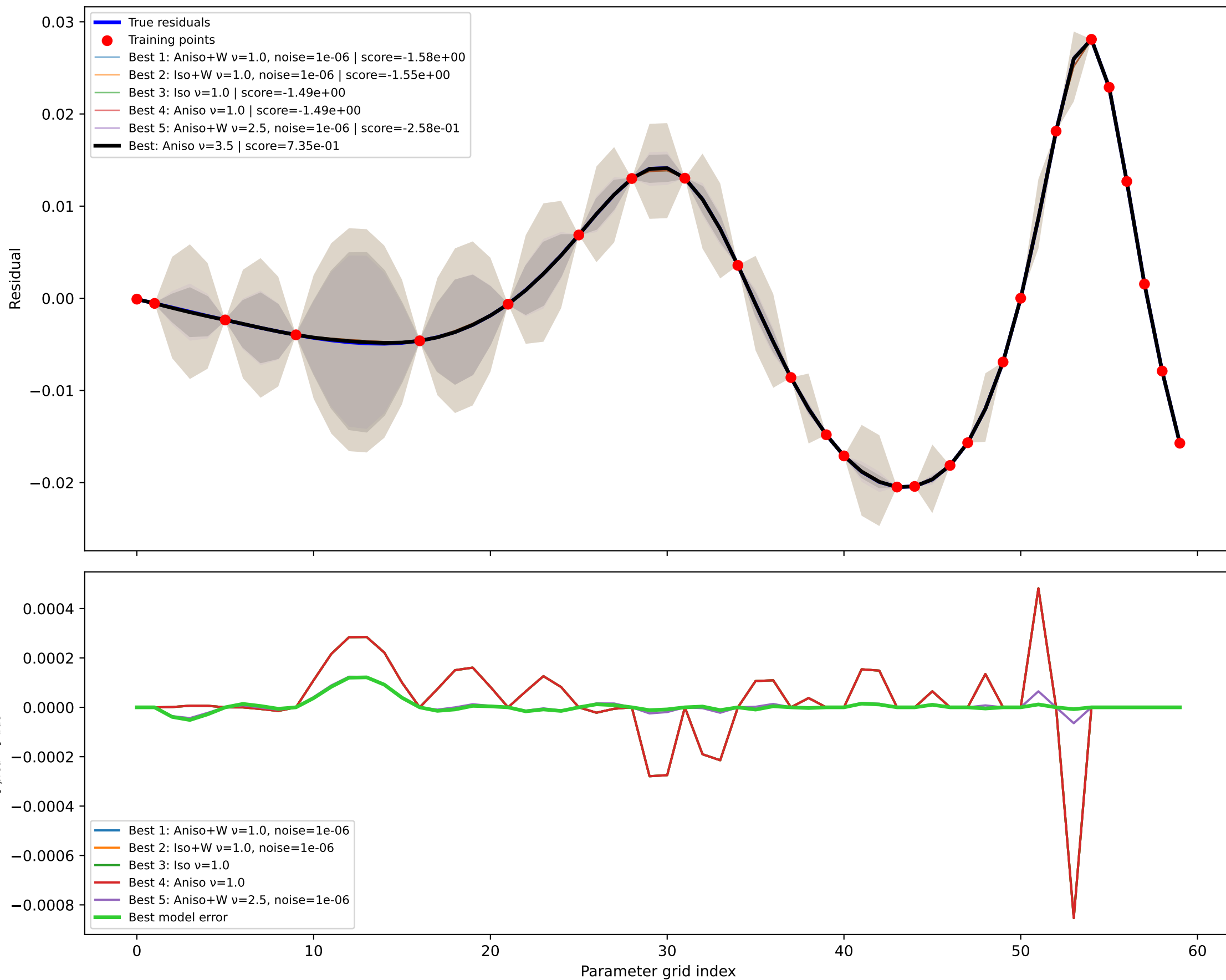
GPR kernel comparison node=6 RMSE=3.024e-05, train RMSE=2.322e-11
